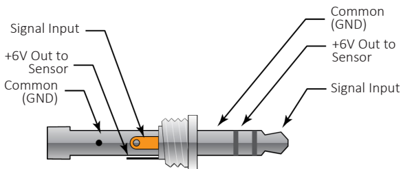
Figure 2 Input Connector Detail (Stereo plug)
